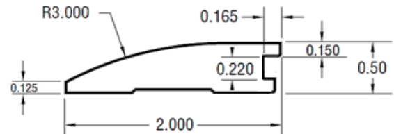
1/2" Reducer
