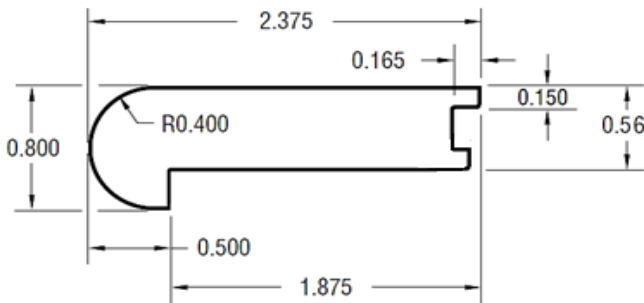
3/8" 1/2" Threshold
