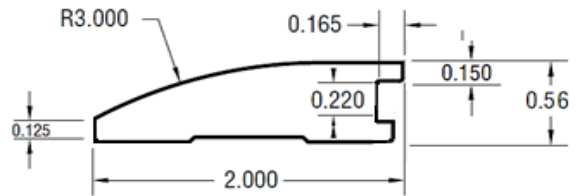
9/16" Reducer
