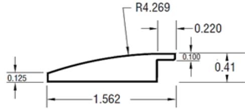
3/8" Reducer
