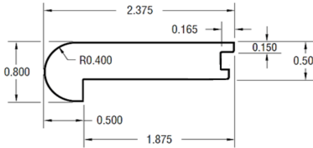
9/16" Stairnose
