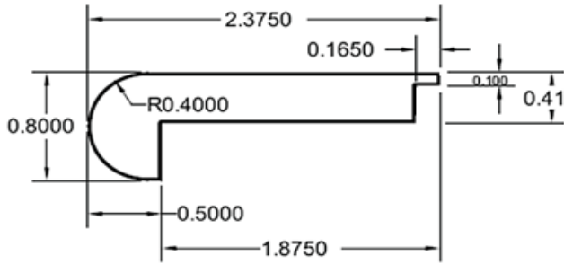
1/2" Stairnose
